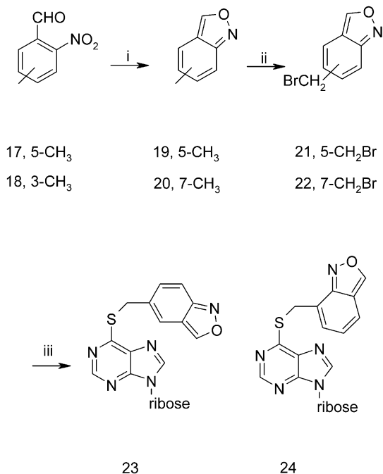
Scheme 2. Preparation of benzisoxazole analogues: (i) SnCl 2 , 2H 2 O, HCl, 15 °C, 2 h; (ii) NBS, Bz 2 O 2 , CCl 4 , N 2 , reflux, 12 h; (iii) 6-mercaptopurine riboside, K 2 CO 3 , DMF, 2 h.
