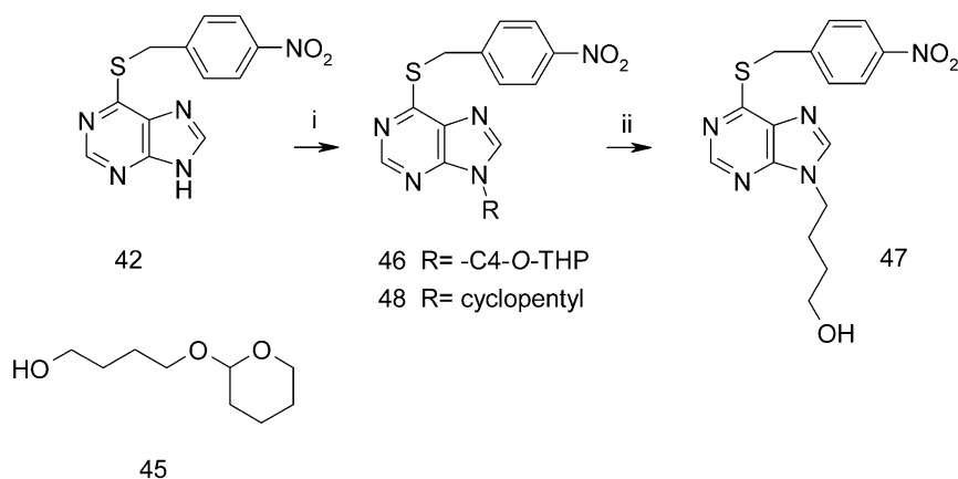
Scheme 7. Synthesis of N9-alkyl-substituted purines via a Mitsunobu reaction: (i) DEAD, PPh 3 , THF (dry), 45 or cyclopentanol; (ii) pTsOH, rt, 2 h.
