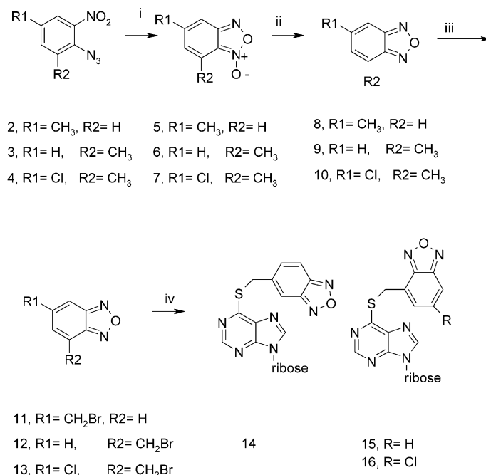
Scheme 1. Preparation of benzofurazan analogues: (i) toluene, reflux, 2 h; (ii) P(OEt) 3 , ethanol, reflux, 30 min; (iii) NBS, Bz 2 O 2 , CCl 4 , N 2 , reflux, 18 h; (iv) 6-mercaptapurine riboside, K 2 CO 3 , DMF, rt.
