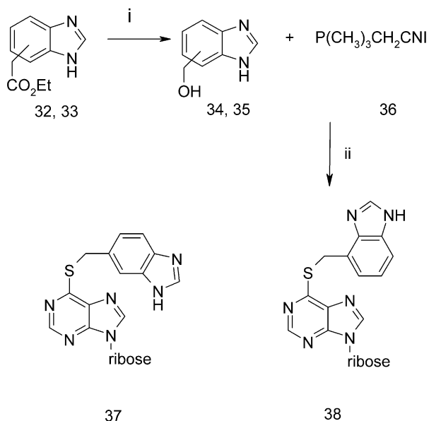
Scheme 4. Preparation of benzimidazole analogues: (i) \text{LiAlH}_4/\text{THF} , 18 h, reflux; (ii) 6-mercaptopurine riboside, DIPEA, propionitrile, reflux, 18 h.
