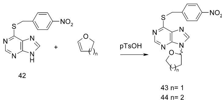
Scheme 6. Synthesis of THF- and THP-protected compounds.
