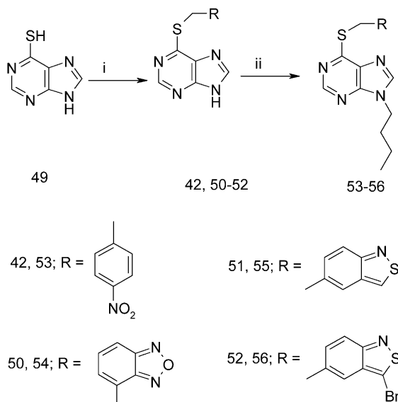
Scheme 8. Synthesis of N9-butylated compounds: (i) appropriate benzyl bromide, K 2 CO 3 , DMF, rt; (ii) NaH, BuBr, DMF, 18 h, rt.
