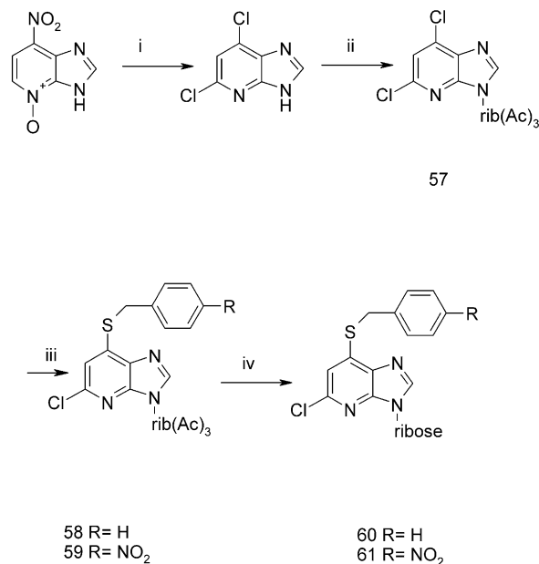
Scheme 9. Synthesis of 2-chloro-1-deaza analogues of NBTI: (i) POCl 3 , DMF; (ii) SnCl 4 , 1,2,3,5-tetra- O -acetyl-β-D-ribofuranose; (iii) 4-nitrobenzylmercaptane, Et 3 N, DMF, rt, 18 h; (iv) NH 3 /CH 3 OH, 0°C.
