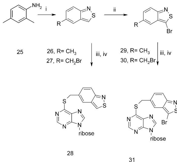
Scheme 3. Preparation of benzoisothiazole analogues: (i) CH 3 SO 2 NSO, benzene (dry), 0 °C to reflux 18 h; (ii) n -BuLi, THF (dry), –78 °C, Br 2 , –78 °C to rt; (iii) NBS, Bz 2 O 2 , CCl 4 , N 2 , reflux, 12 h; (iv) 6-mercaptopurine riboside, K 2 CO 3 , DMF, 2 h.
