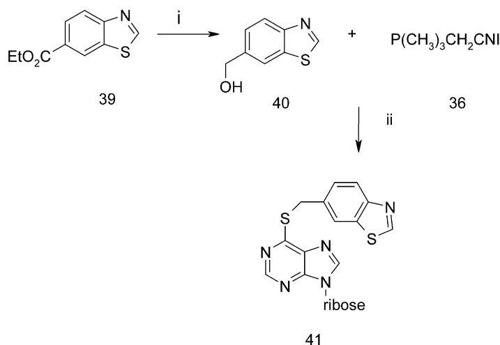
Scheme 5. Preparation of benzothiazole analogues: (i) \text{LiAlH}_4/\text{THF} , 18 h; (ii) 6-mercaptopurine riboside, DIPEA, propionitrile, reflux, 18 h.
